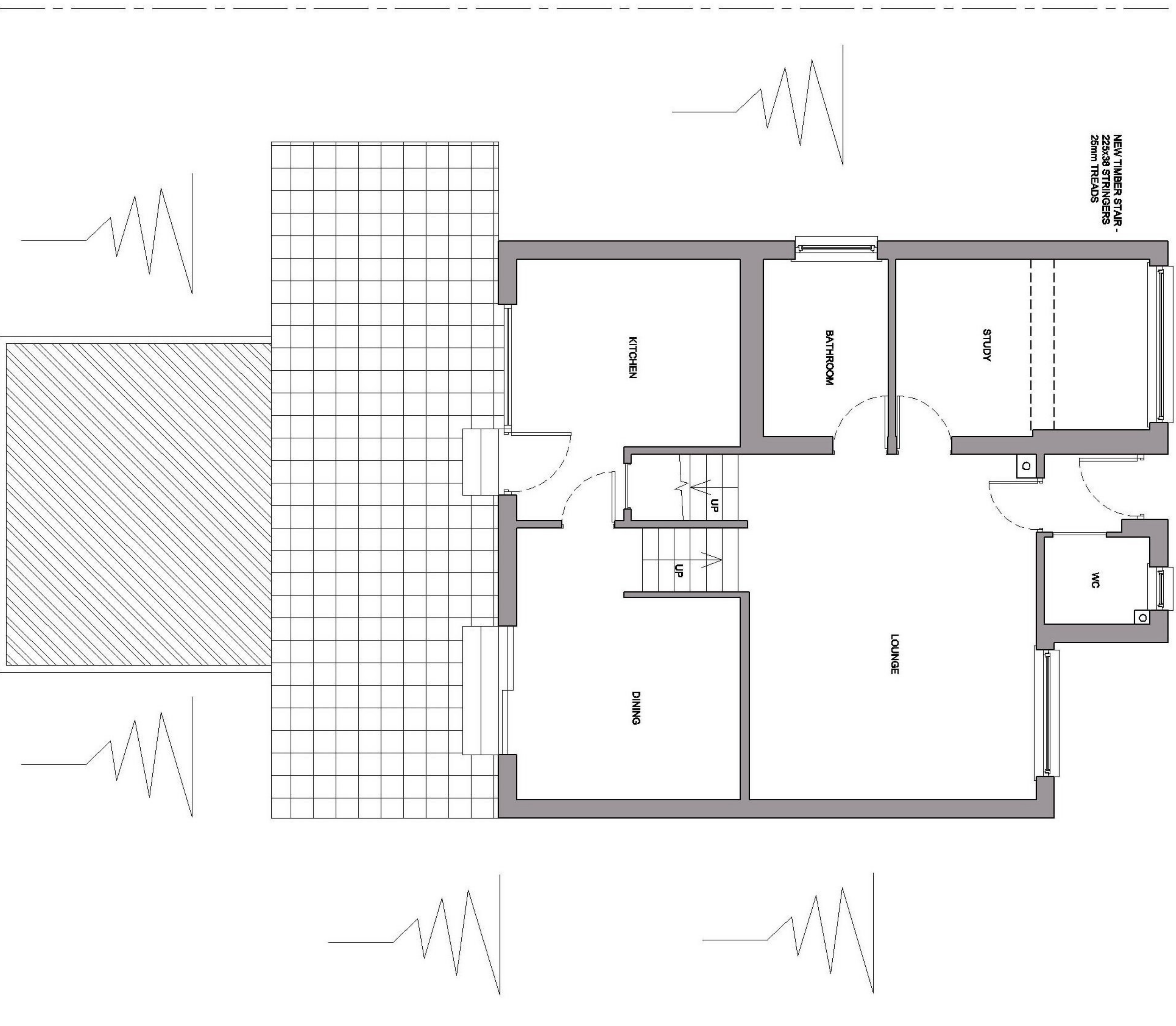
1:50 LOWER UPPER GROUND FLOOR WALL LAYOUT AS EXISTING
