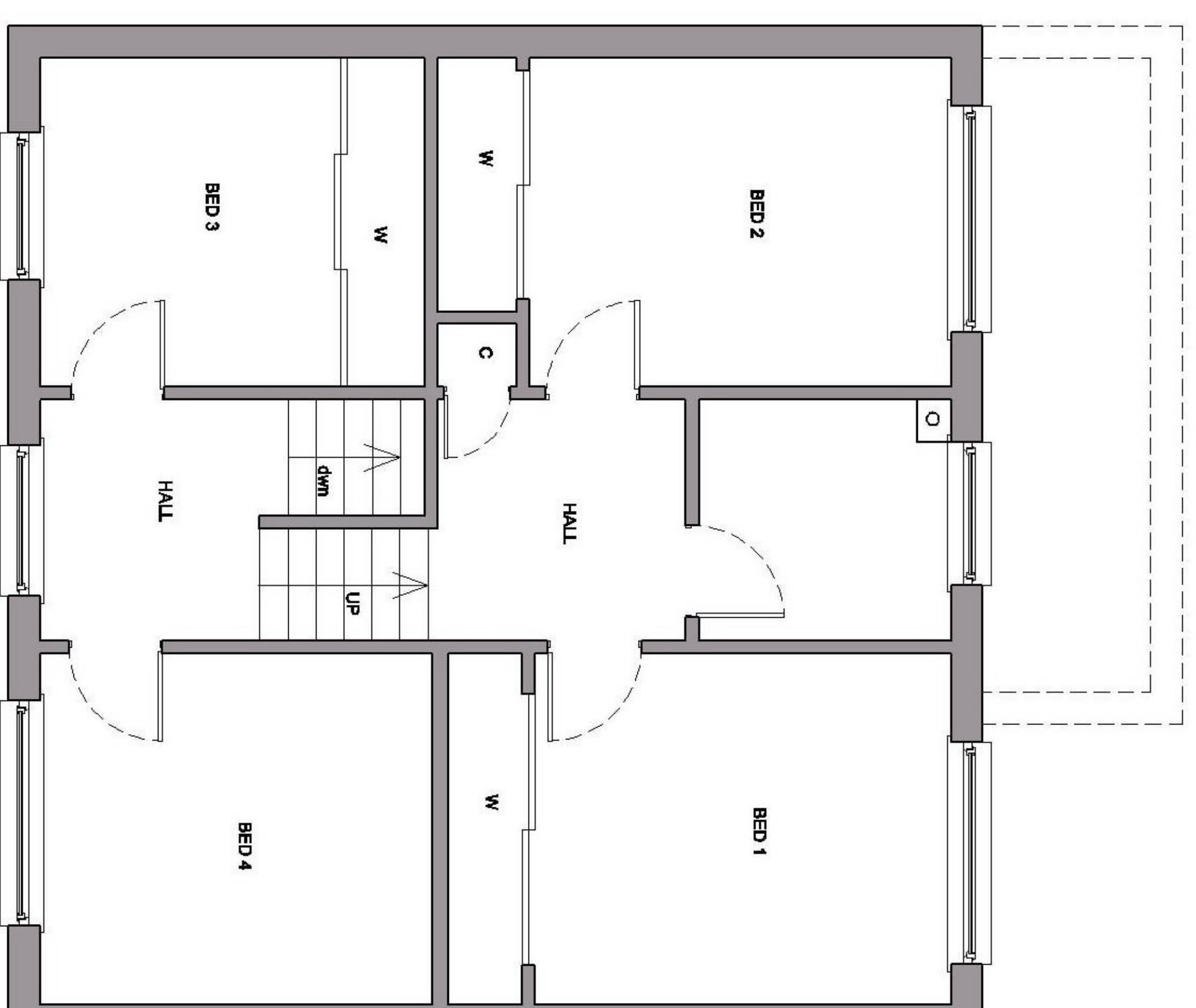
1:50 LOWER UPPER FIRST FLOOR WALL LAYOUT AS EXISTING
