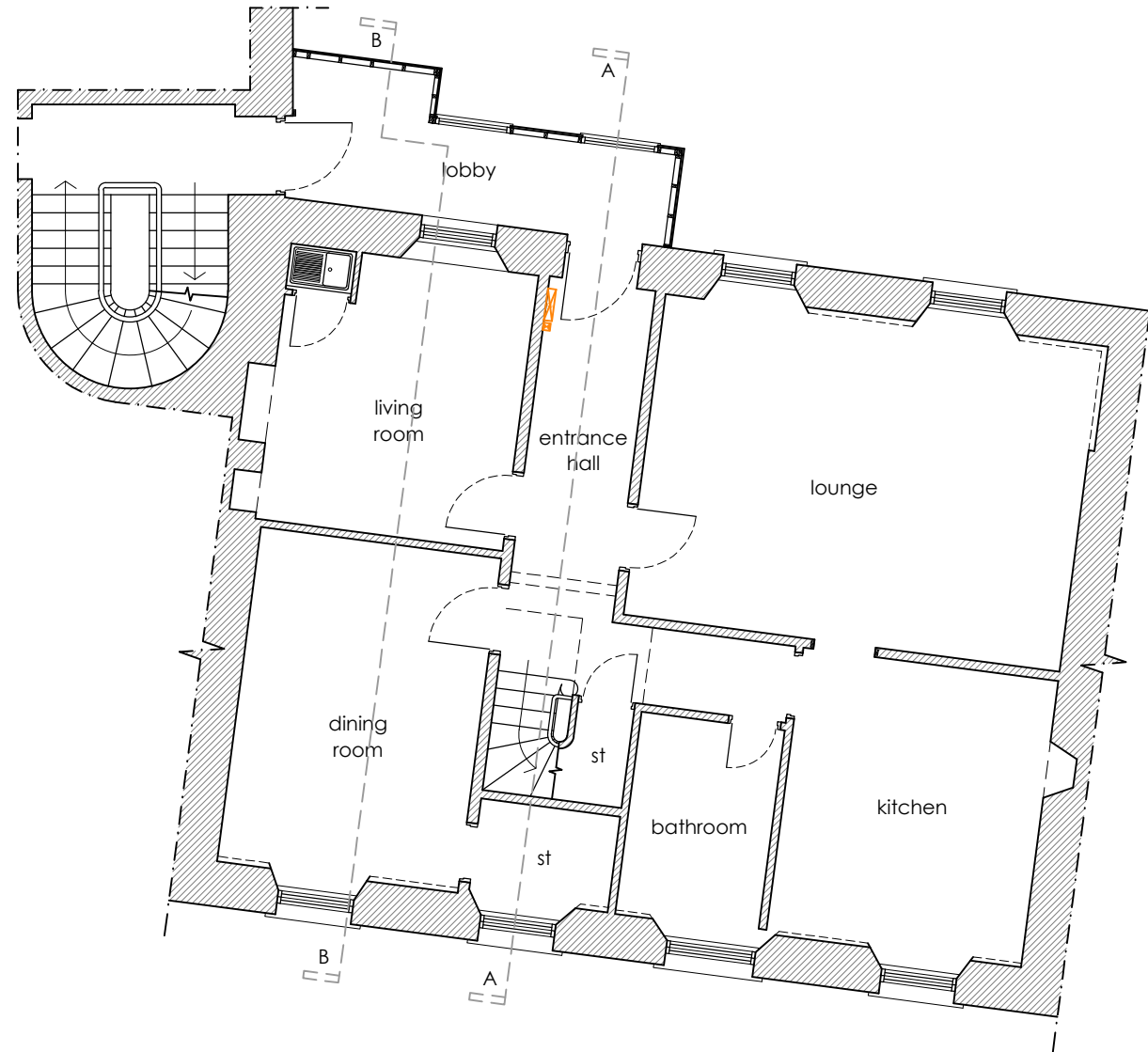
Existing Lower Floor Plan (second floor) 1/100 @ A3
