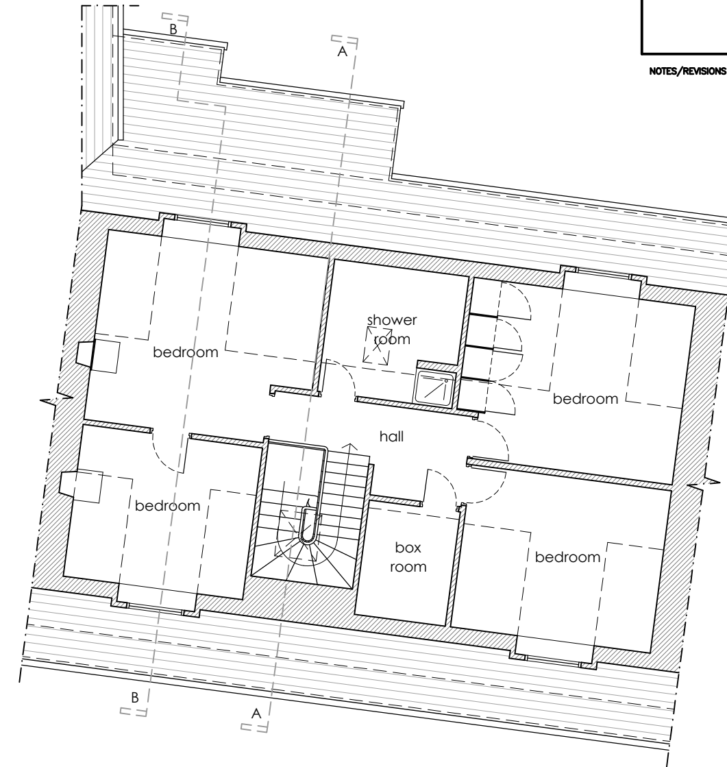
Existing Upper Floor Plan (third floor) 1/100 @ A3
