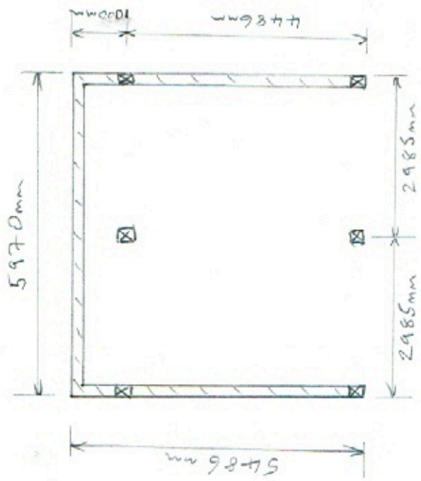
CART LODGE FLOOR PLAN (SCALE 1:100)
