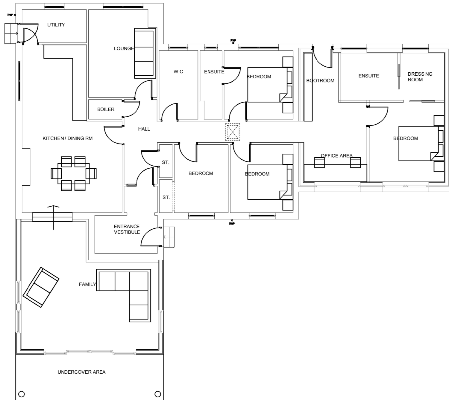
PROPOSED GROUND FLOOR PLAN 1:100 @ A3
