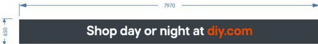
Sign: 03 - scale 1:50 1-OFF Shallow folded aluminium panelling painted dark grey with self coloured vinyl text applied to face. Sign installed to cladding area below main sign.
