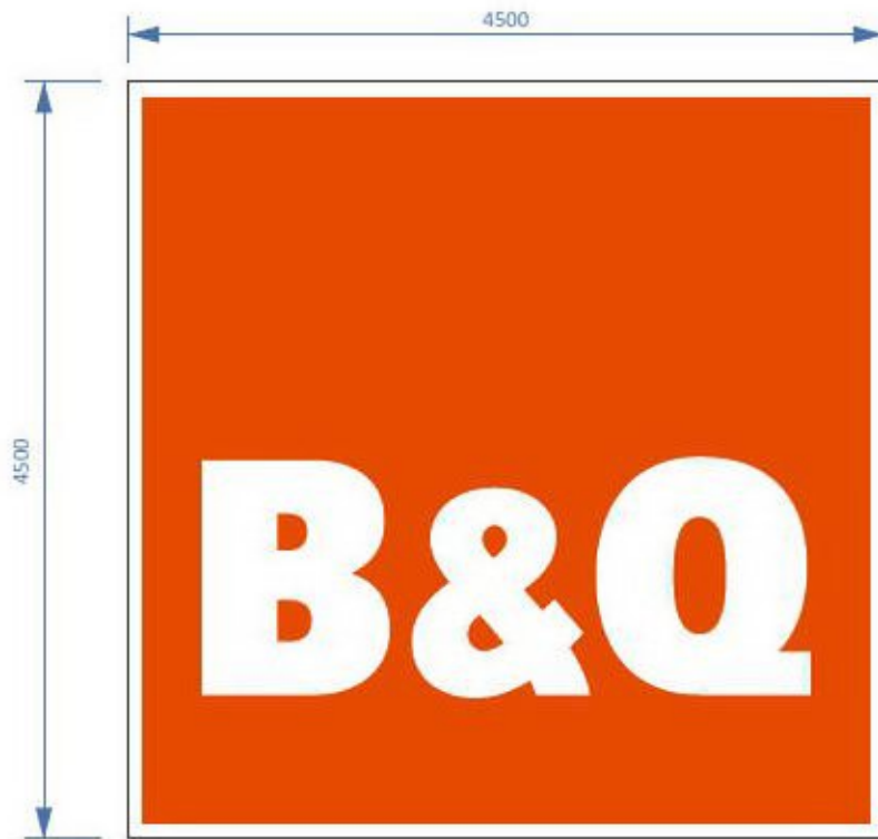
Sign: 01 - scale 1:50 1-off 4.5m sq. Signcase with orange returns c/w vinyl decorated flex skin. Full internal illumination with static LED Note: support frame maybe require subject to site survey
