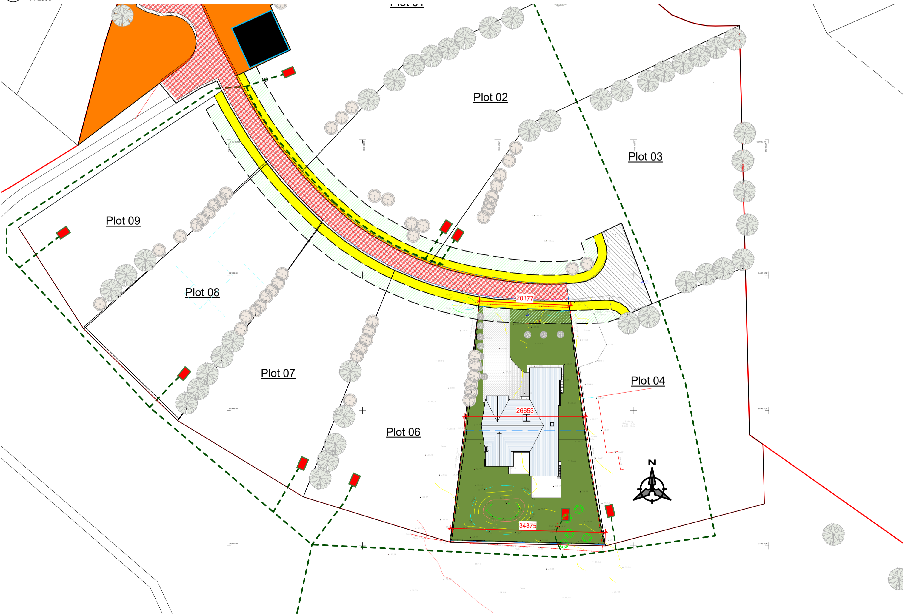
2 Proposed Block Plan 1:500
