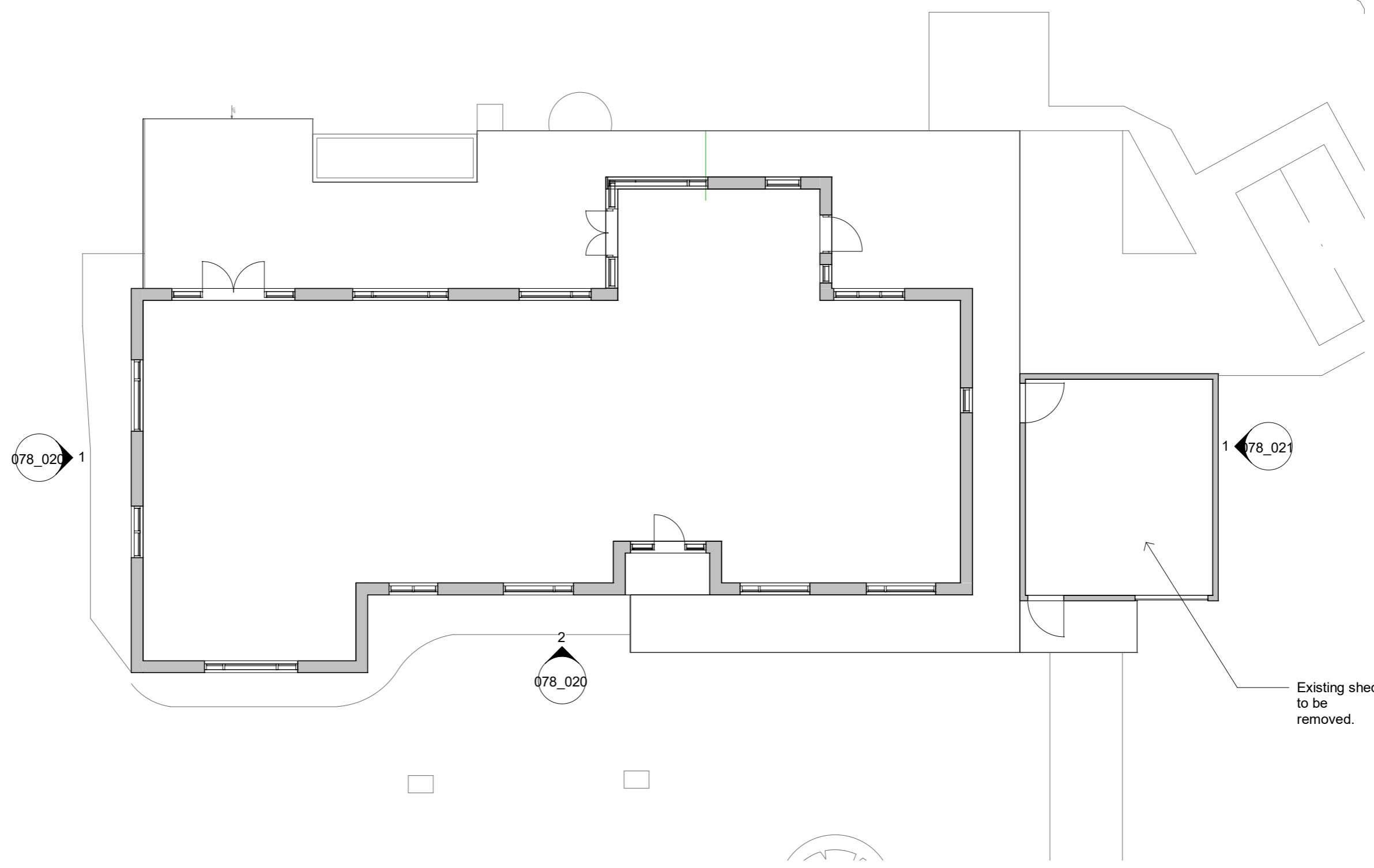
1 Existing Ground floor plan 1 : 100
