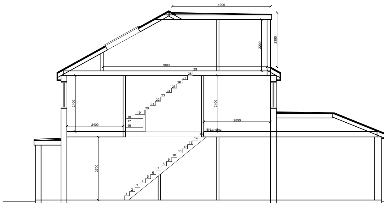
EXISTING SECTION
