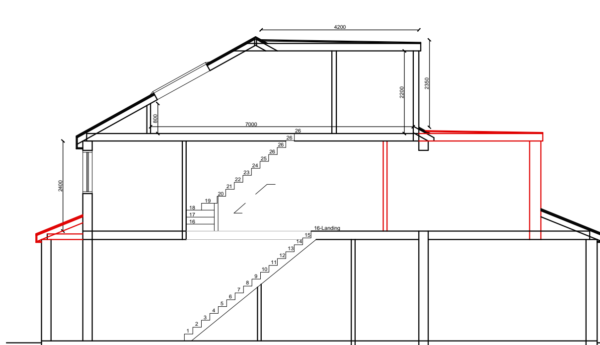
PROPOSED SECTION
