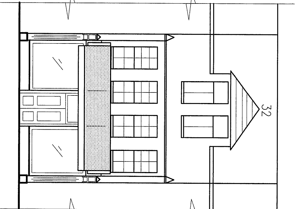
FRONT ELEVATION
