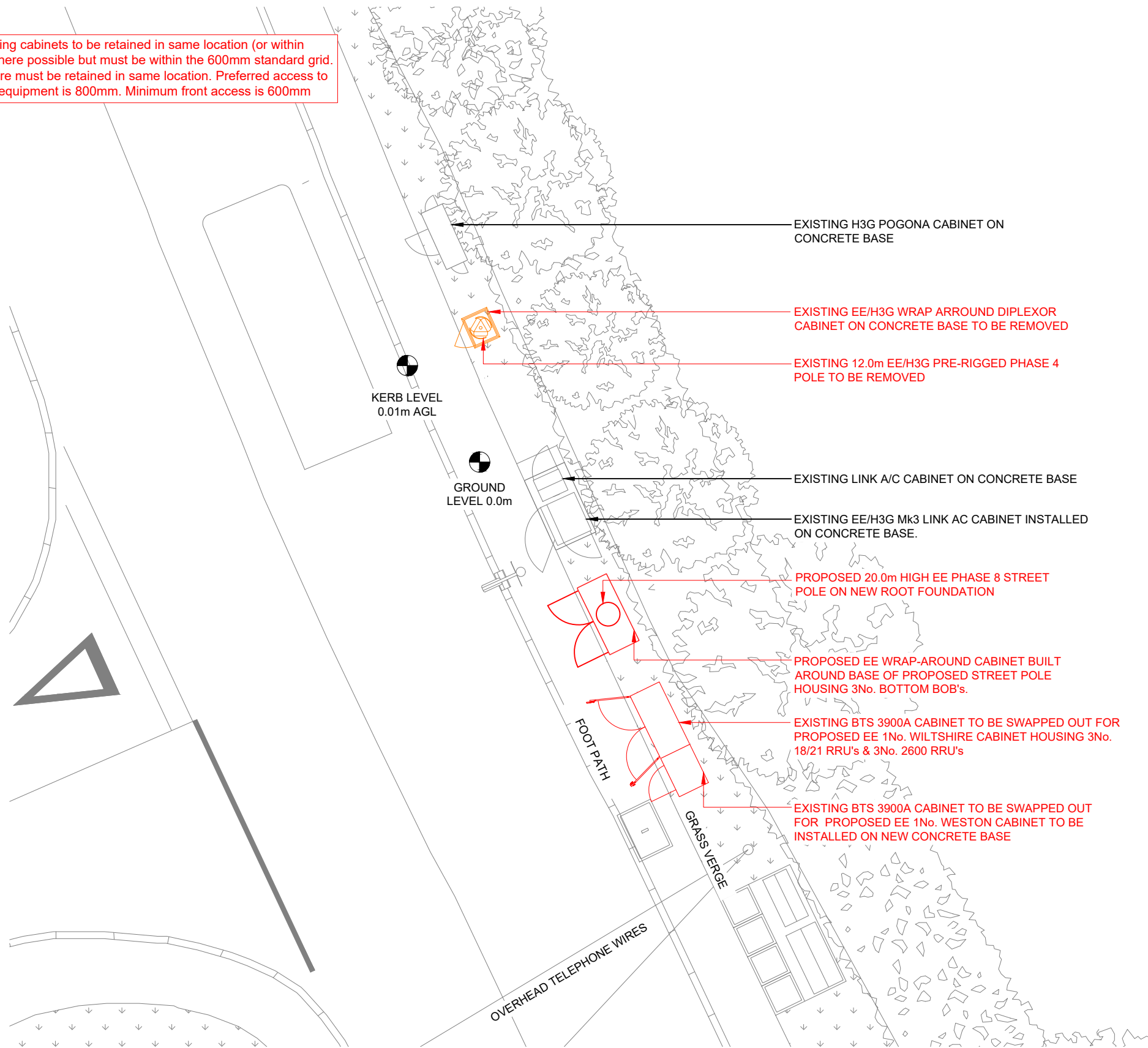
PROPOSED SITE LAYOUT
