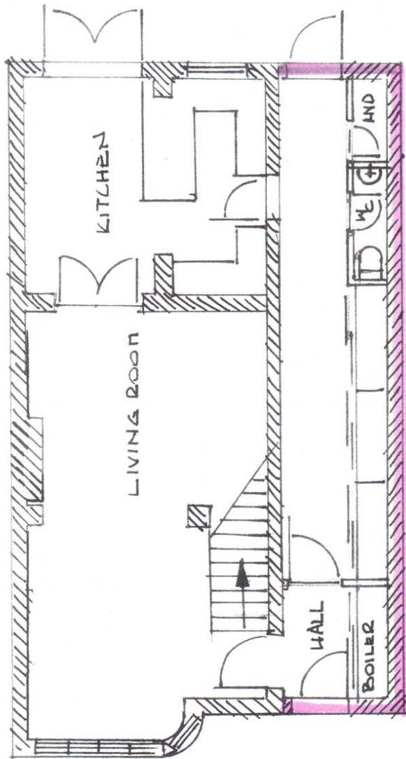
GROUND FLOOR - PROPOSED
