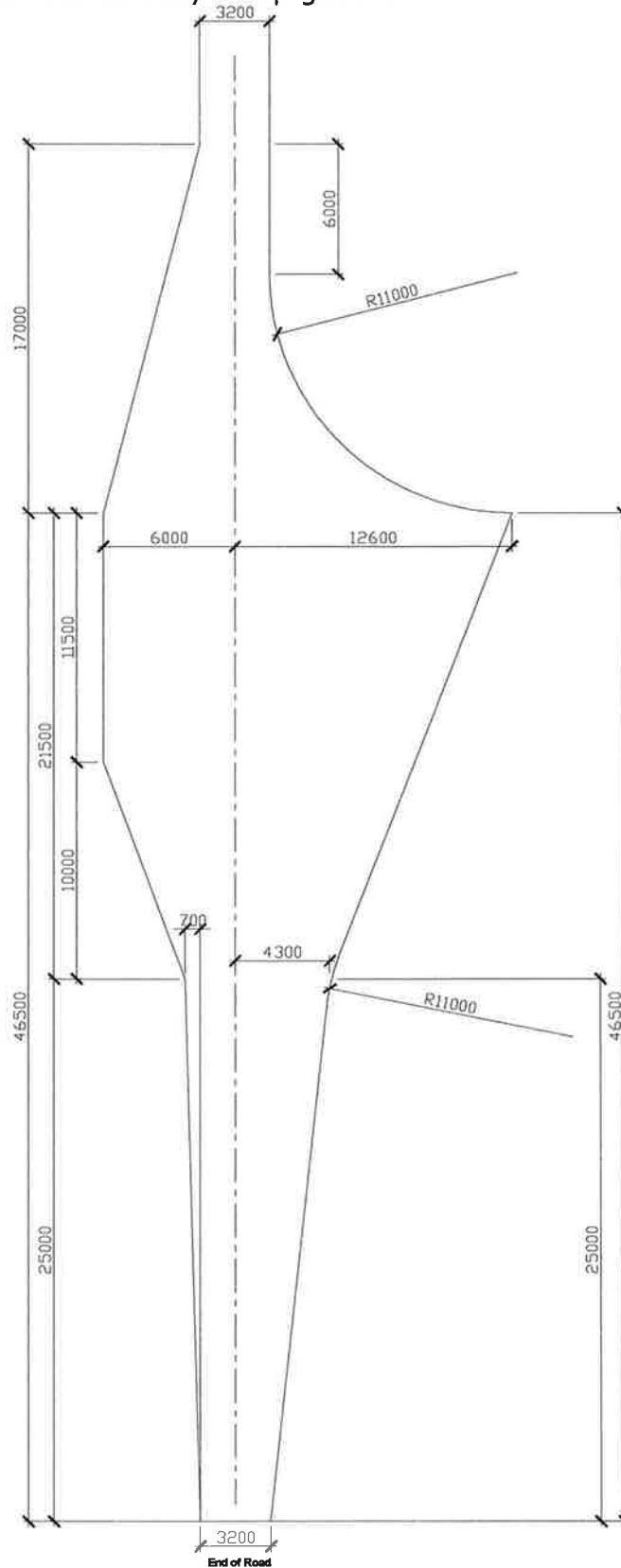
Figure 8 Turning point for road on very steep ground
