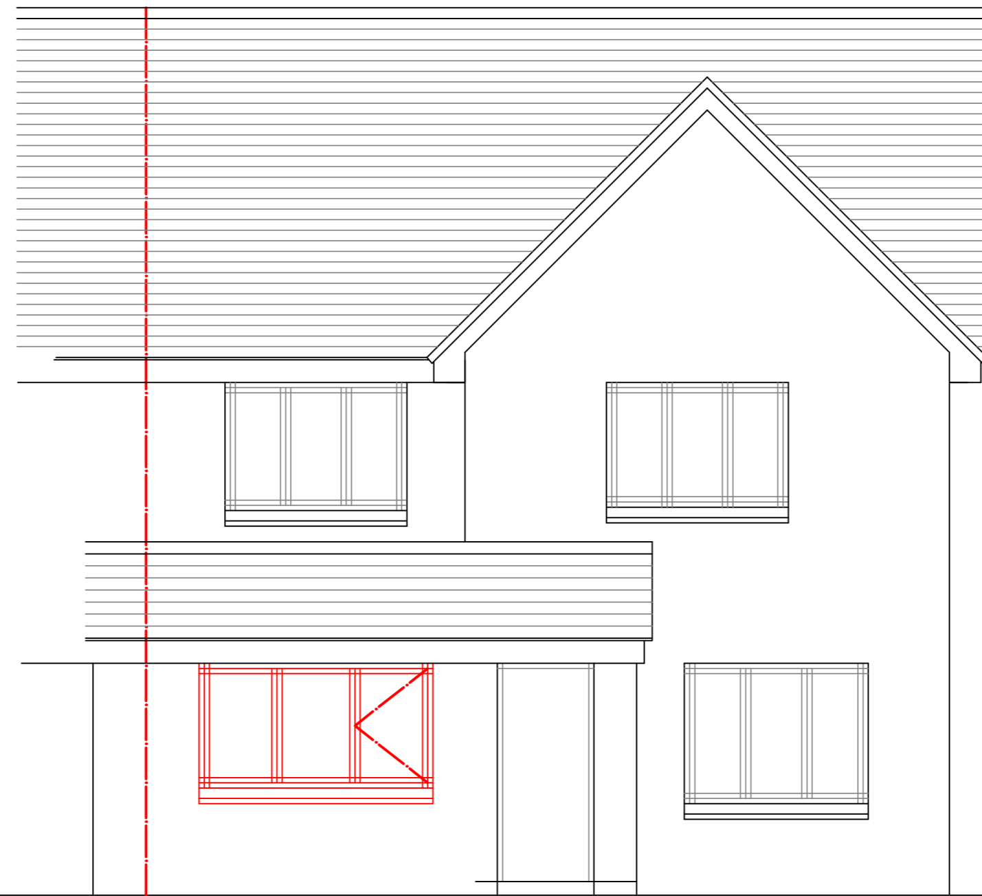
FRONT ELEVATION
