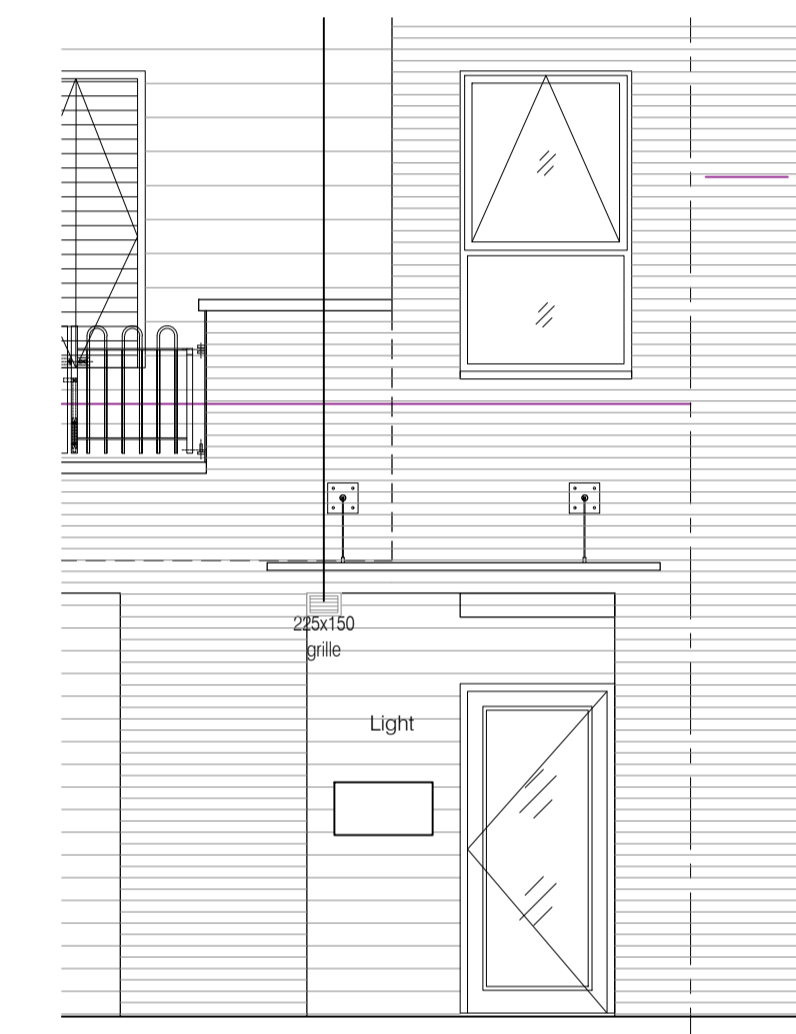
Enlarged Elevation pt2- Scale - 1:50
