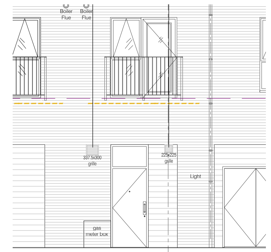
Enlarged Elevation pt3- Scale - 1:50
