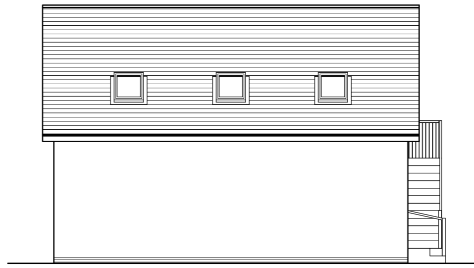
REAR ELEVATION
