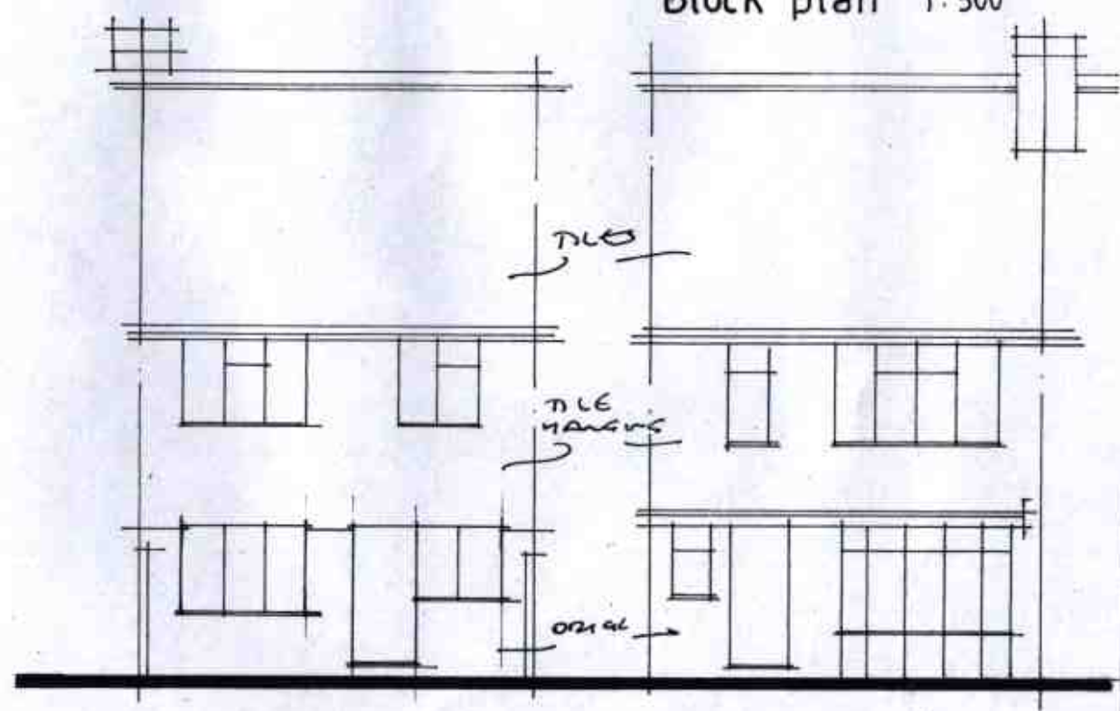
Existing East 1:100 West
