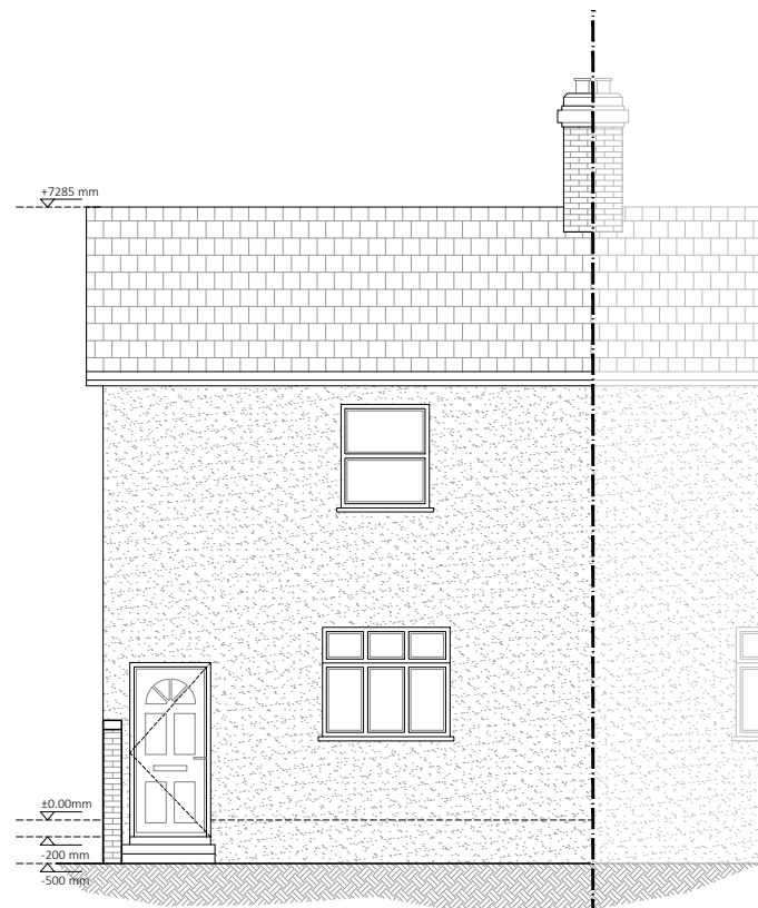
EXISTING SOUTHWEST ELEVATION
