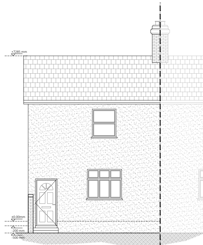
PROPOSED SOUTHWEST ELEVATION (NO CHANGES)
