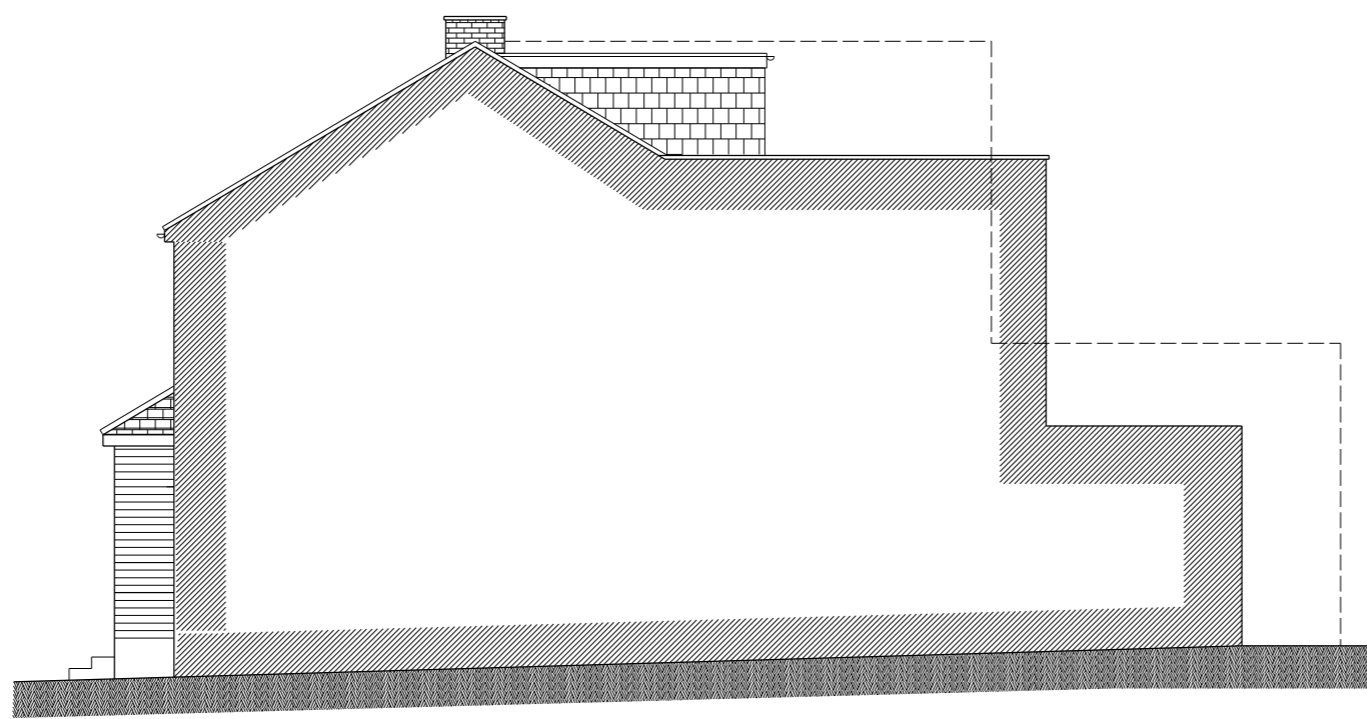
Existing No. 67 Side Elevation (1:100)
