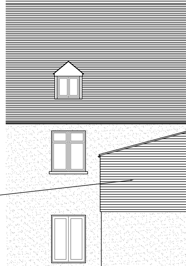
Proposed South-East Elevation
