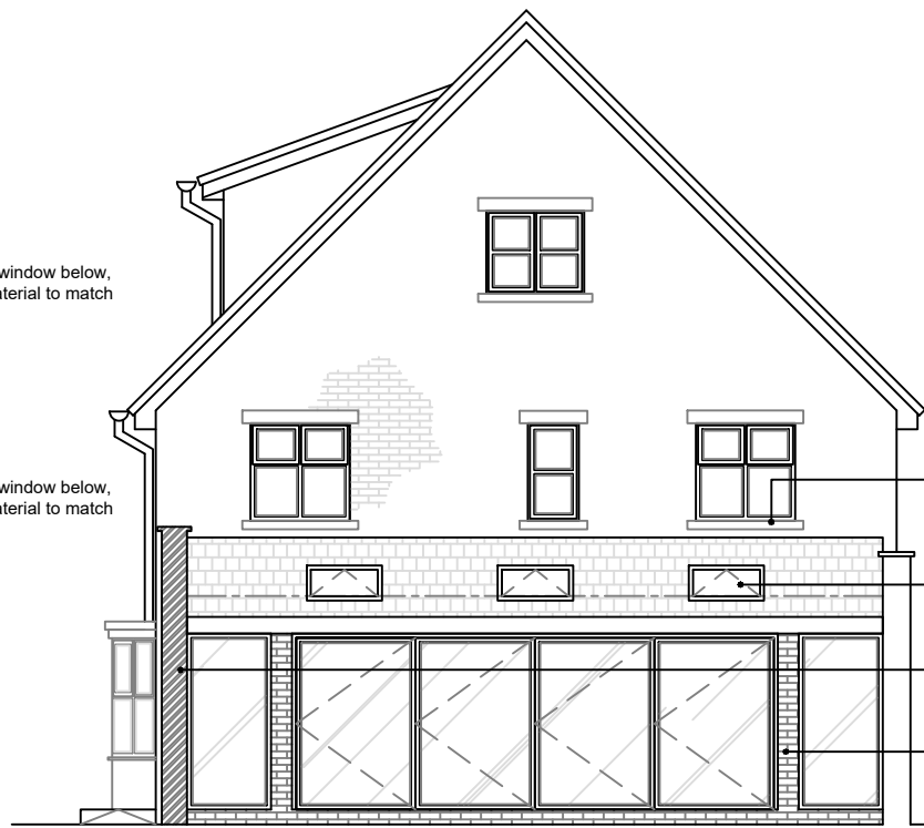
Proposed R/H Side Elevation 1:100
