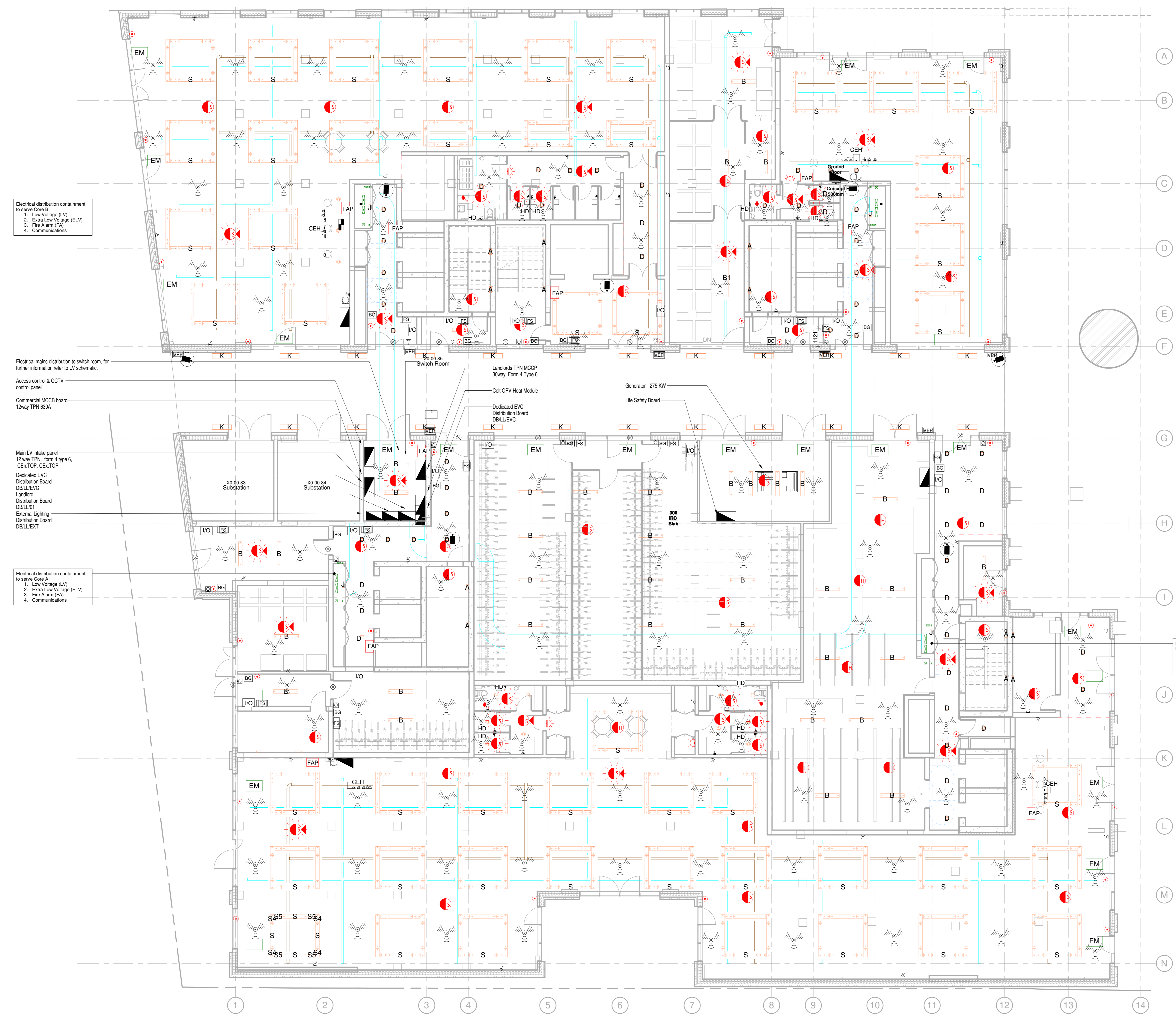
1 LEVEL 00 - Electrical Services 1 : 100
