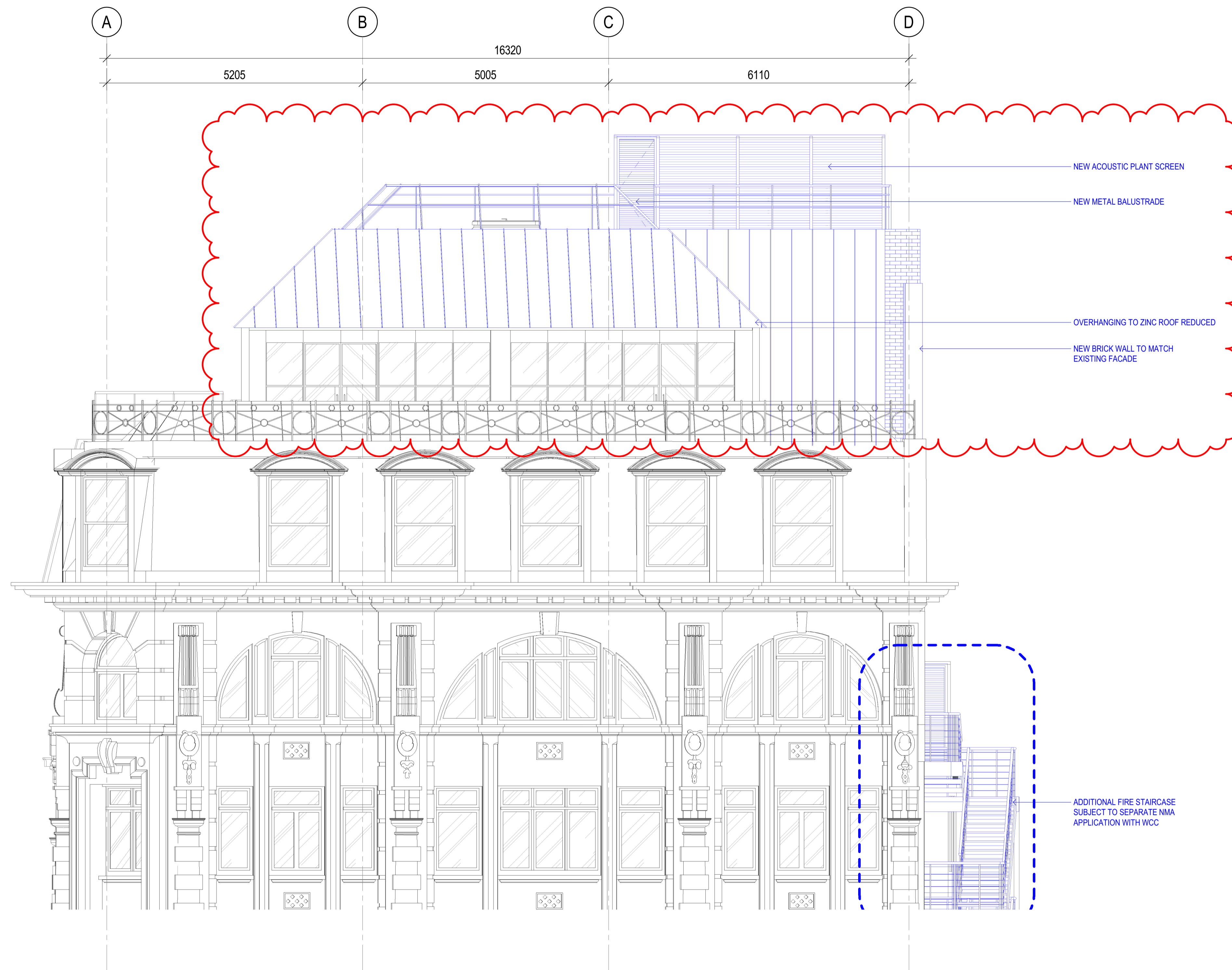
1 Proposed Roof Extension Elevation (SOUTH EAST) ELEVATION 1:50
