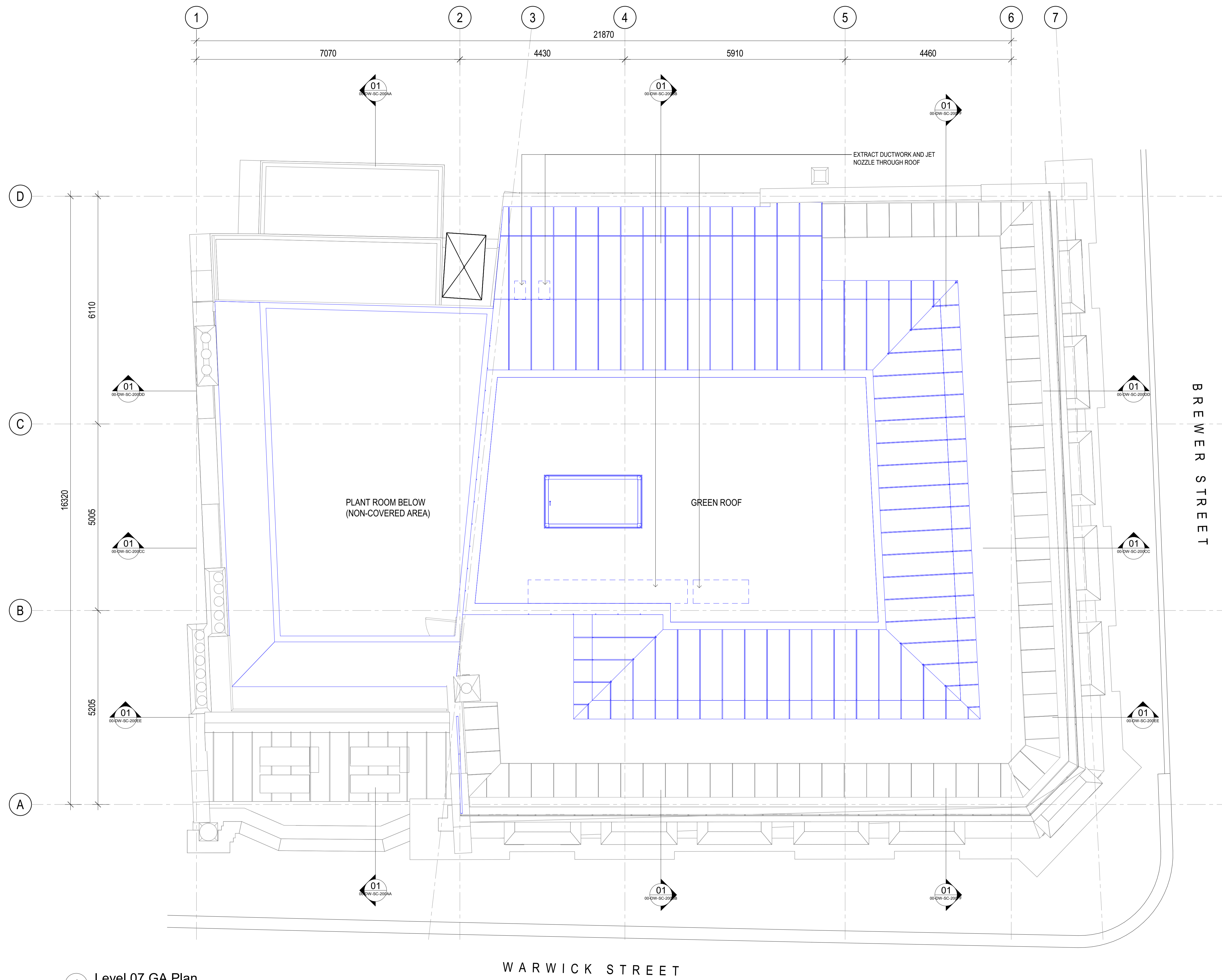
1 Level 07 GA Plan PLAN 1:50
