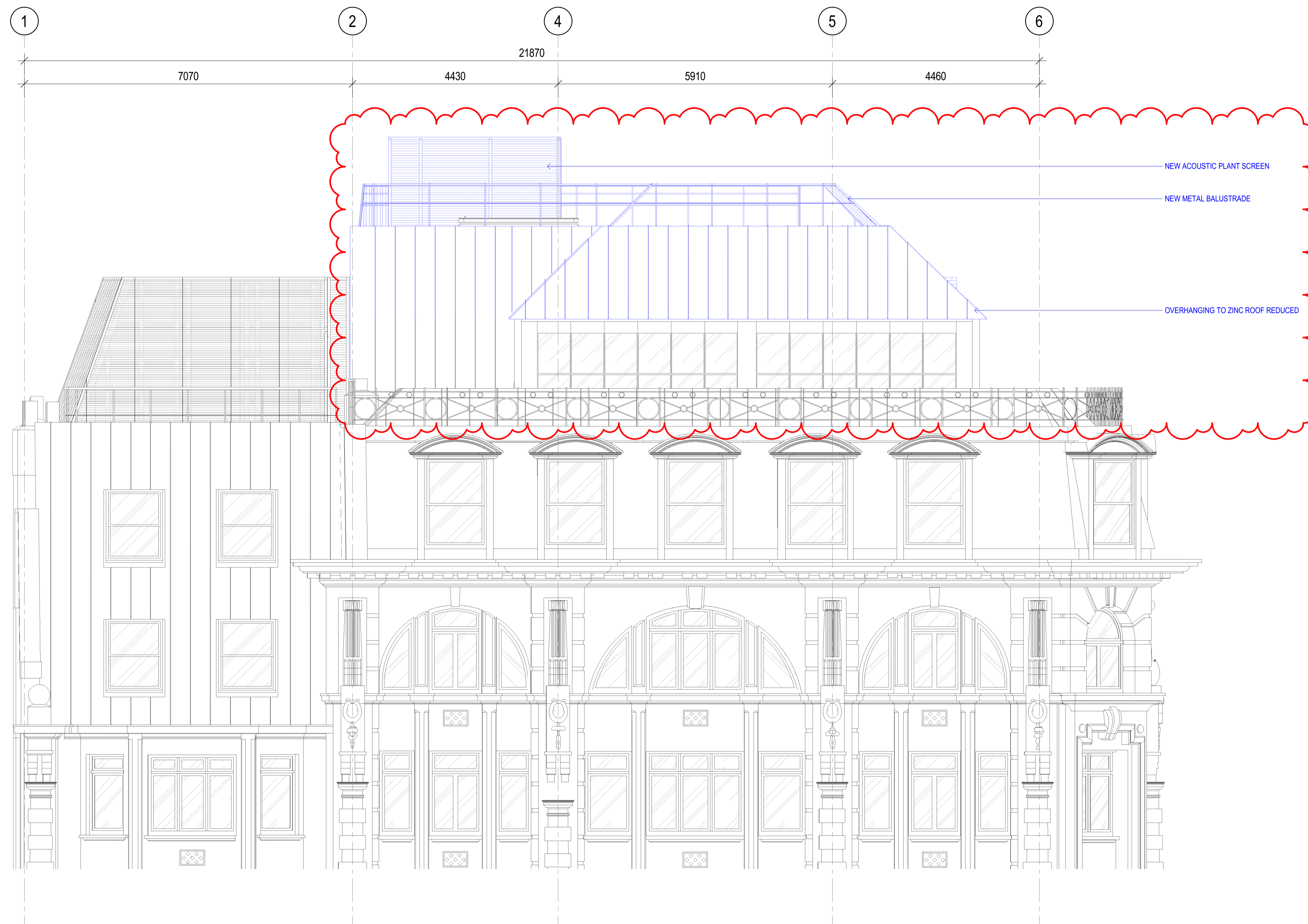
1 Proposed Roof Extension Elevation (SOUTH WEST) ELEVATION 1:50
