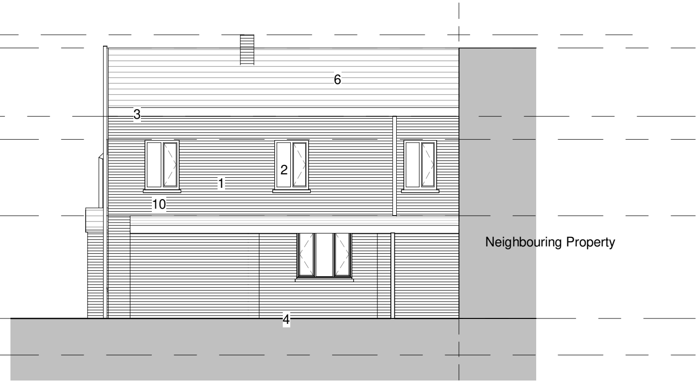
South East Elevation - As Existing 1 : 100
