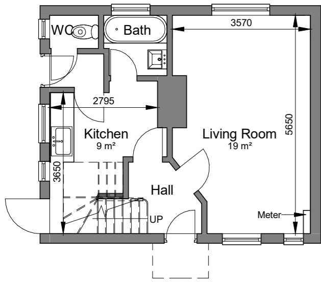
1 Ground Floor Plan 1 : 100
