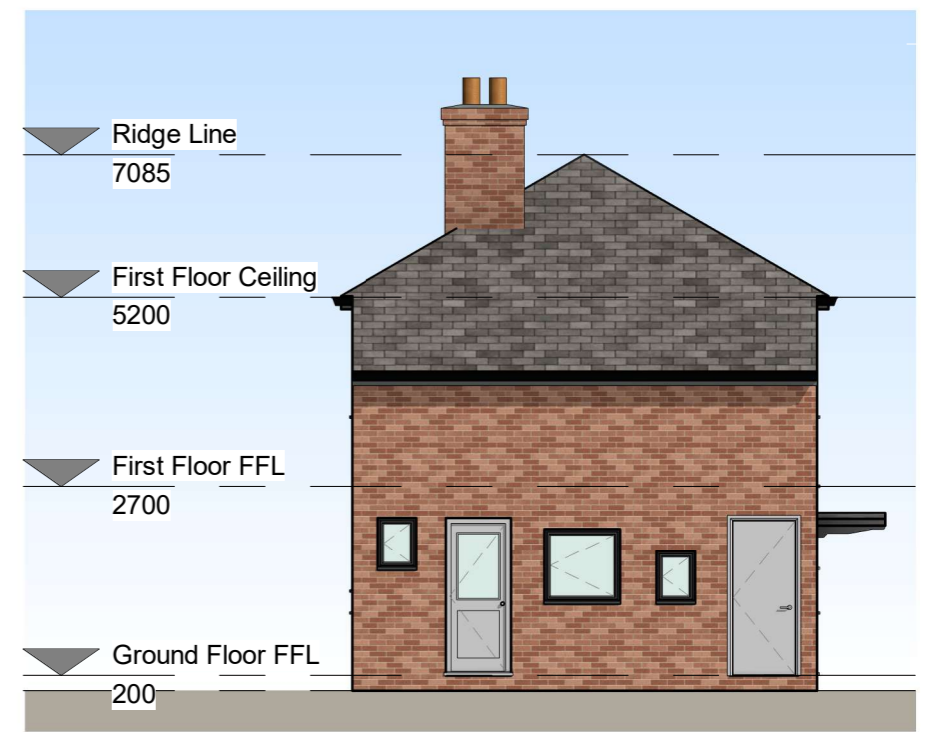
7 04 - Side Elevation 1 : 100
