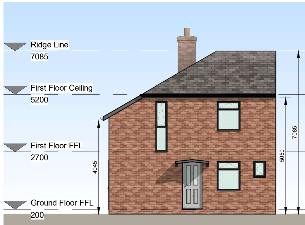
4 Front Elevation 1 : 100
