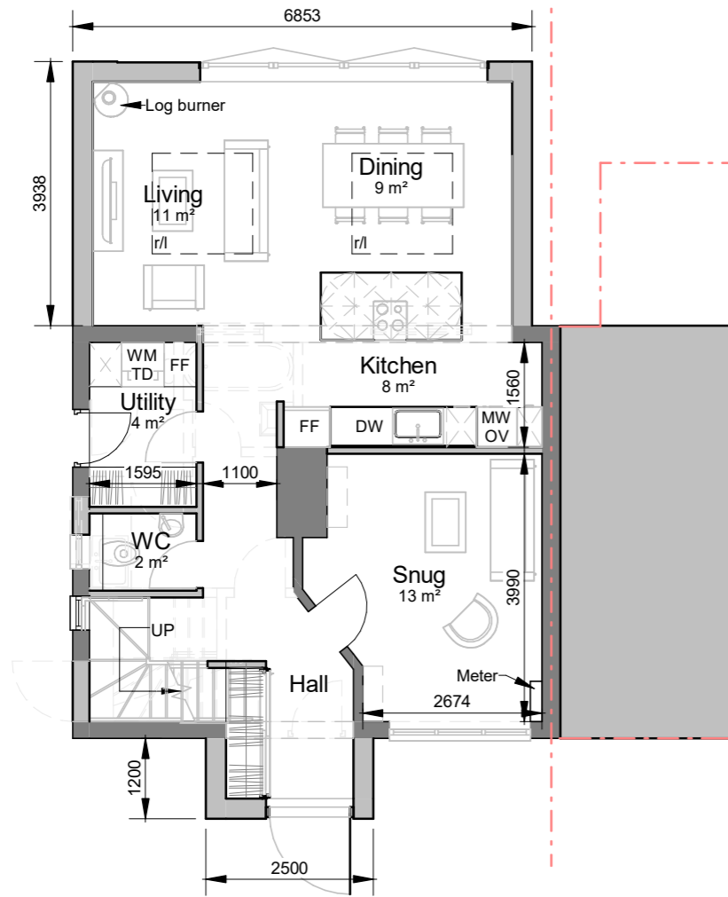
1 Ground Floor Plan 1 : 100
