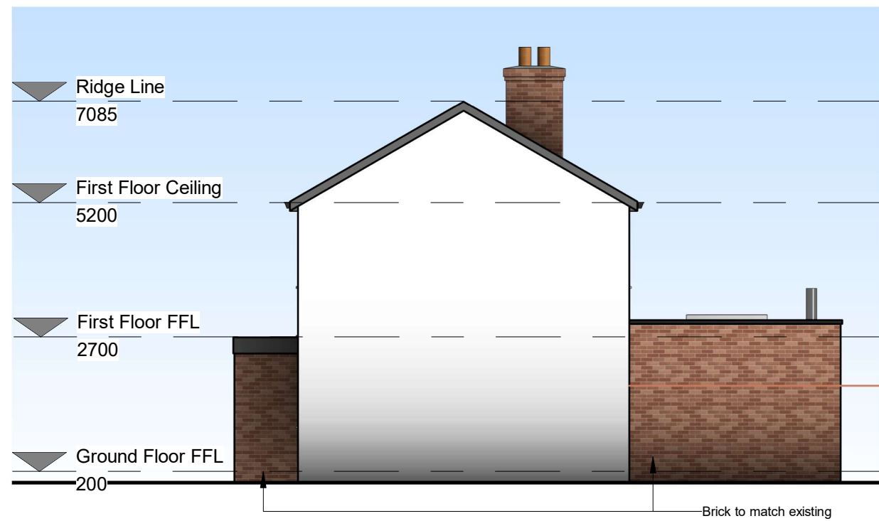
3 Side Elevation 1 : 100
