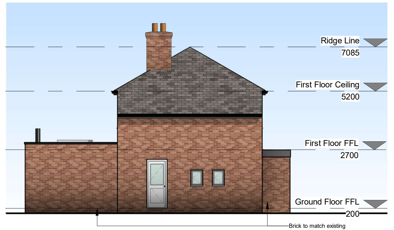
4 Side Elevation 1 : 100
