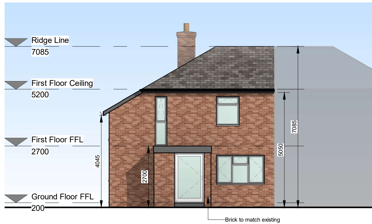
1 Front Elevation 1 : 100
