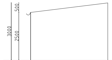
NORTHEAST ELVATION
