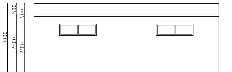
NORTHWEST ELEVATION
