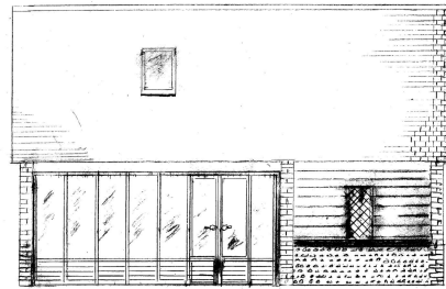
SOUTH ELEVATION SCALE 1/50
