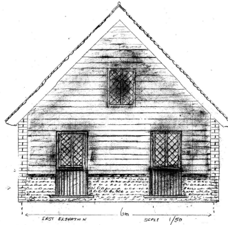
EAST ELEVATION SCALE 1/50
