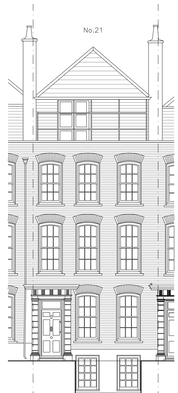
Existing Front Elevation 1:100
