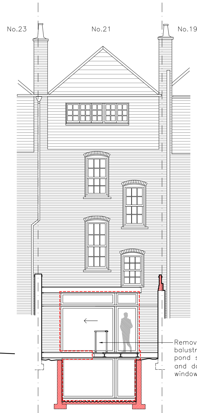
Existing Section B-B 1:100
