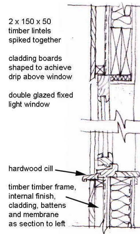
window cill and head detail 1:10
