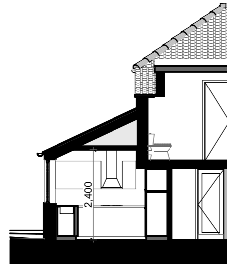
Section CC 1:100
