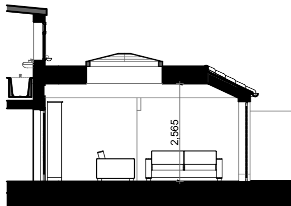
Section AA 1:100
