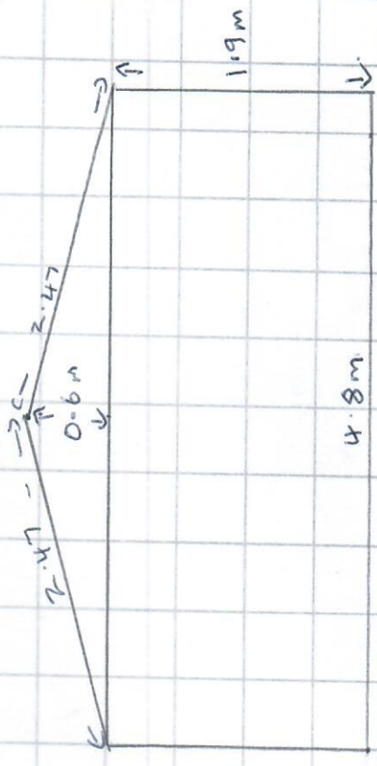
Shed end elevation (R.H.S. from Doggetts Barn)
