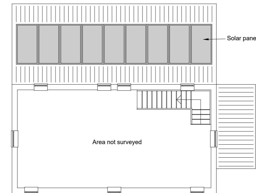
Proposed First Floor Plan @ 1:100
