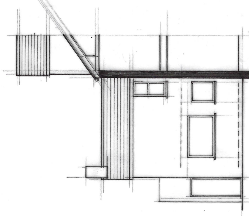
EXIST. NORTH ELEVATION
