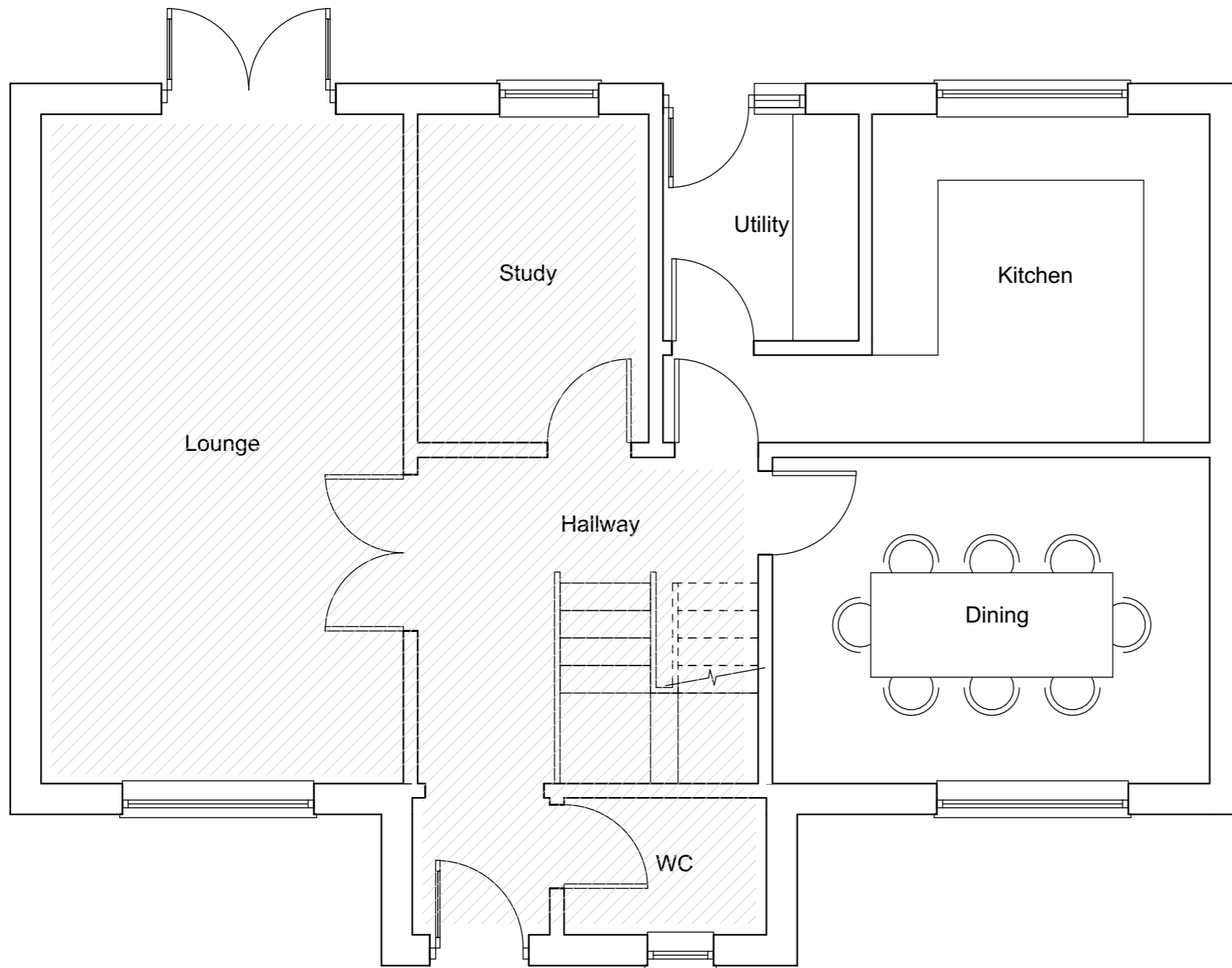
Ground Floor Plan as Existing 1:50
