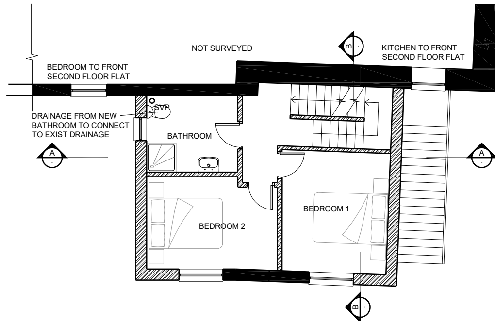
SECOND FLOOR AS PROPOSED
