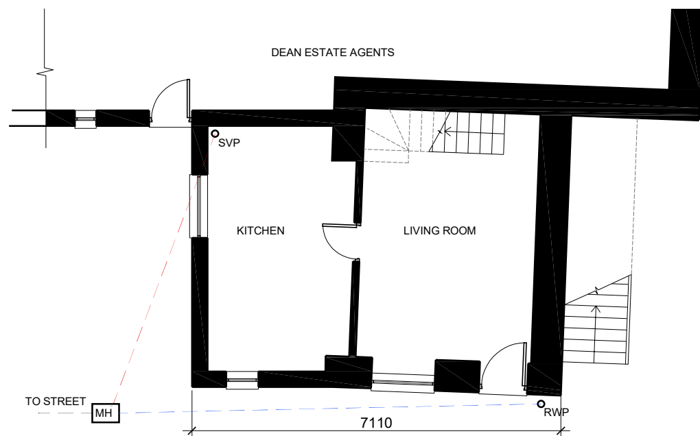
GROUND FLOOR AS PROPOSED (NO CHANGE)
