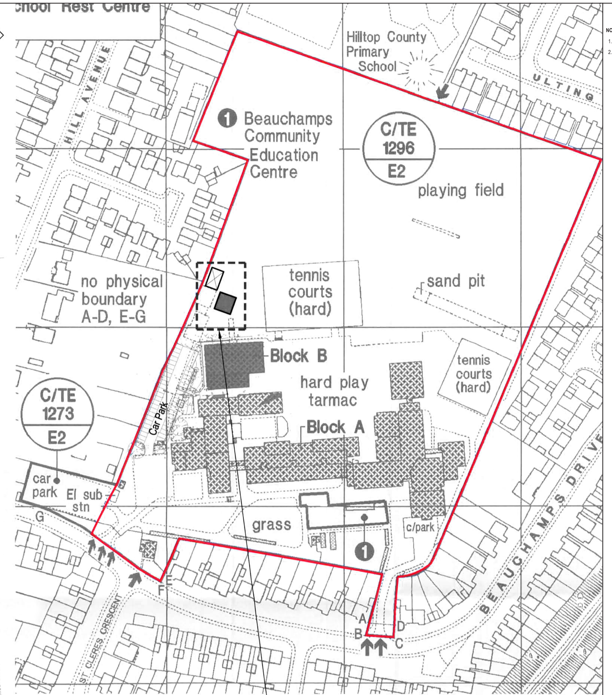
LOCATION PLAN Scale 1:1250 0 10m 50m 100m 5m 20m
