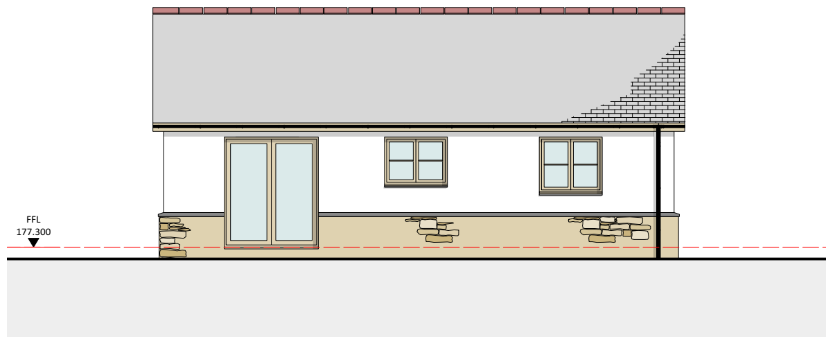
3 SOUTH-EAST ELEVATION SCALE: 1:100
