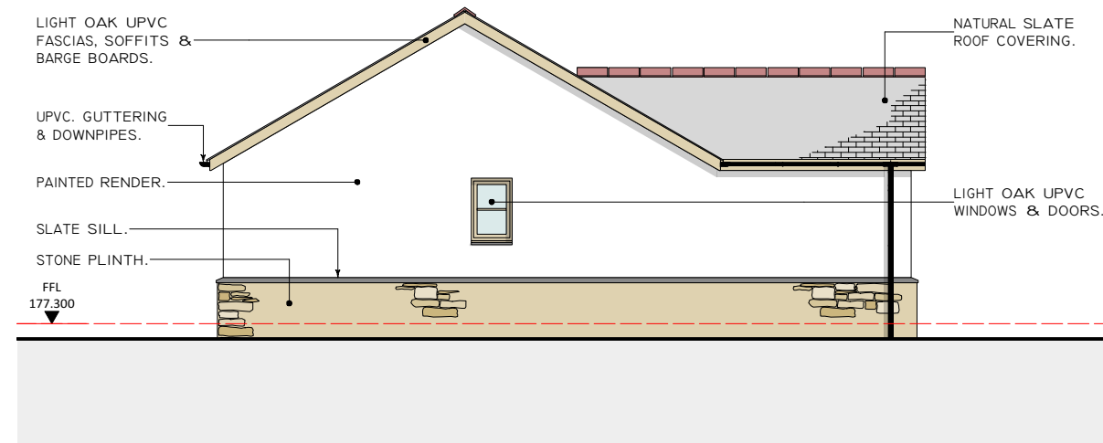
2 NORTH-EAST ELEVATION SCALE: 1:100
