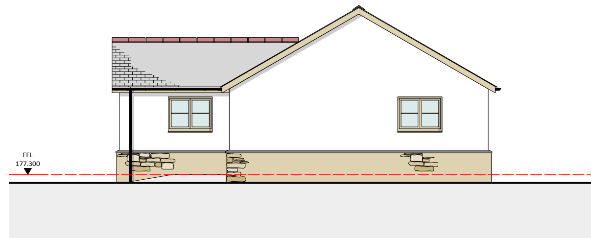
4 SOUTH-WEST ELEVATION SCALE: 1:100
