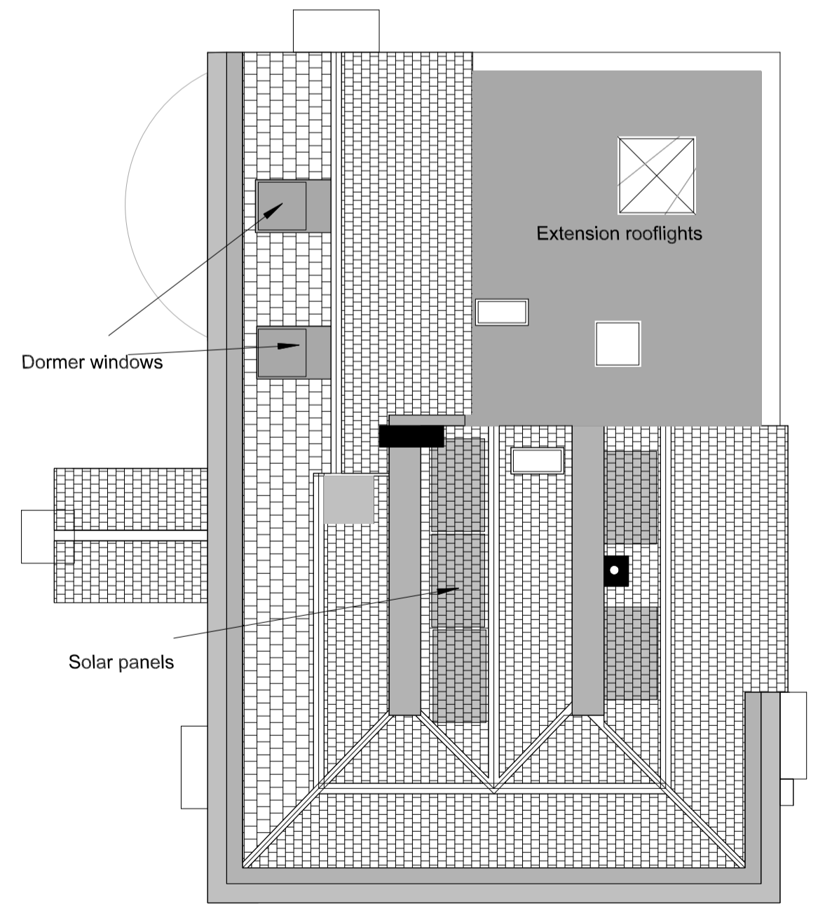
Proposed Roof arrangements
