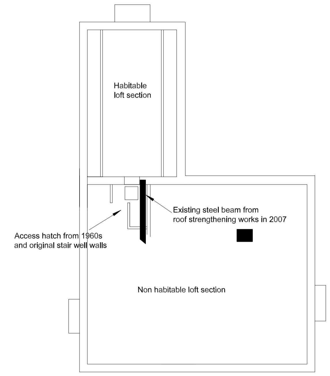
Existing Loft level
