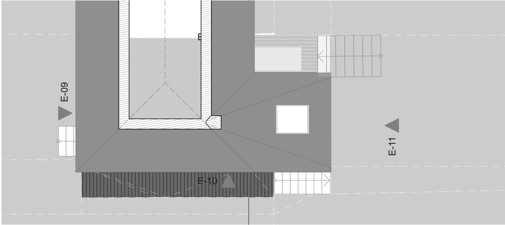
BVN.04.2 PROPOSED ROOF PLAN 1:100
