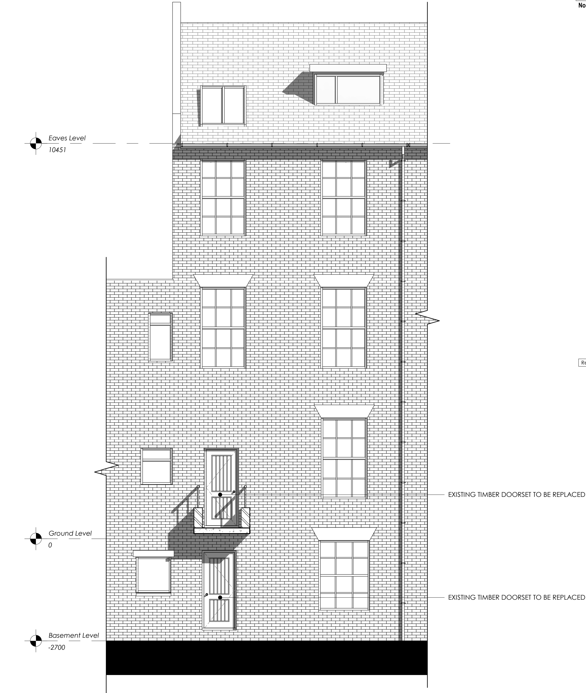
1 Rear Elevation 1 : 50
