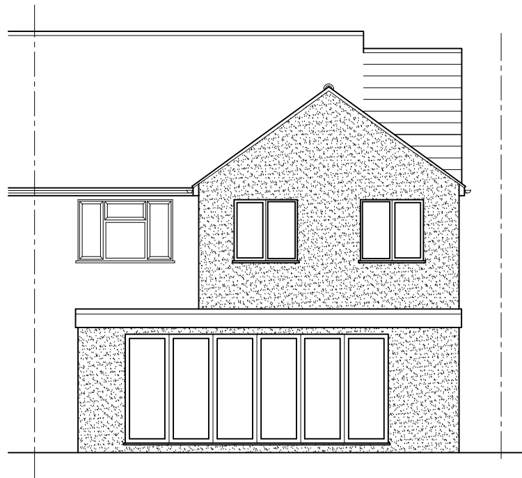
PRE EXISTING REAR ELEVATION
