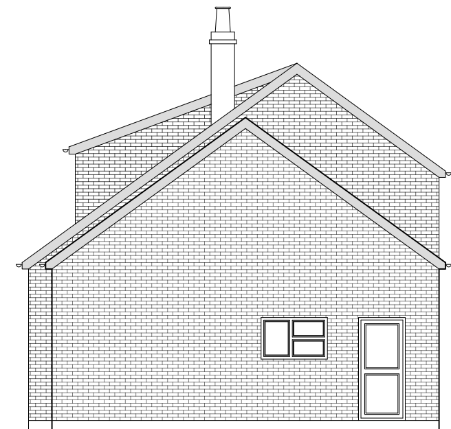
EAST ELEVATION 1:100
