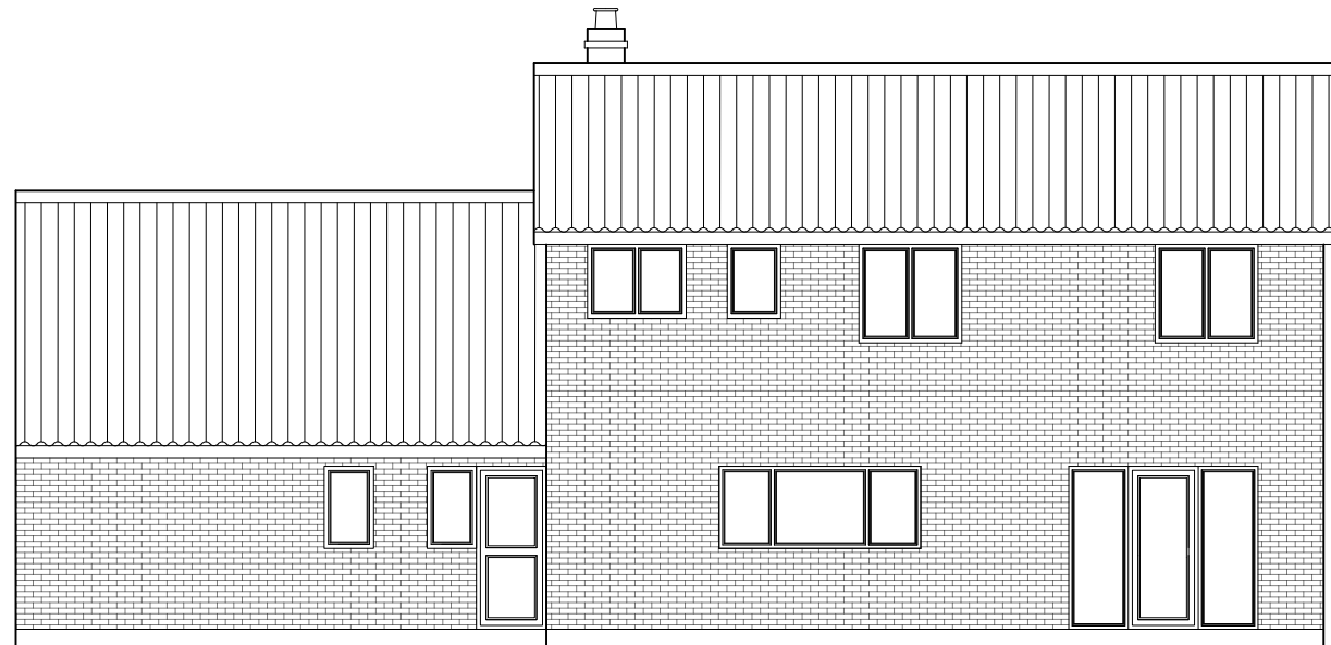
NORTH ELEVATION 1:100
