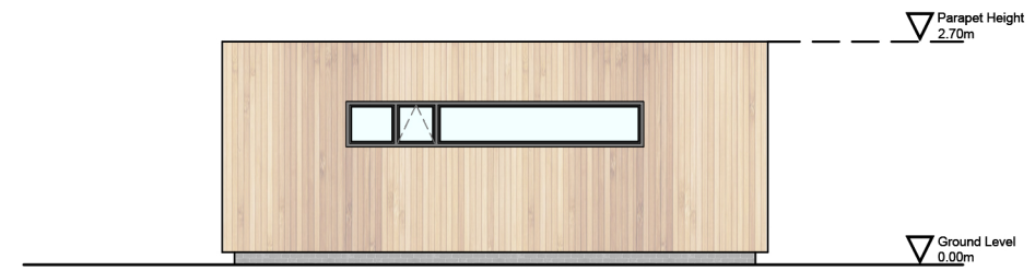
EAST ELEVATION 1:100
