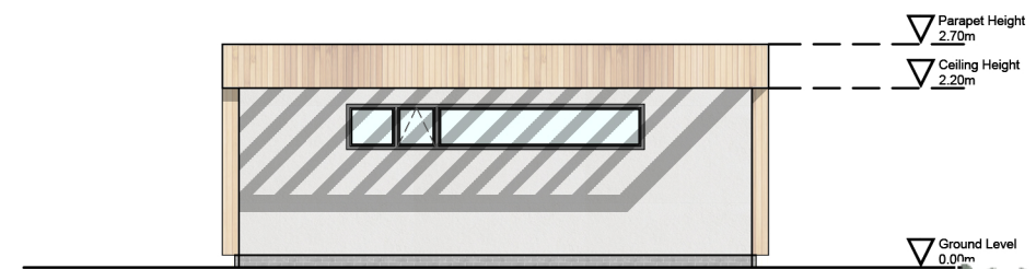
WEST ELEVATION 1:100
