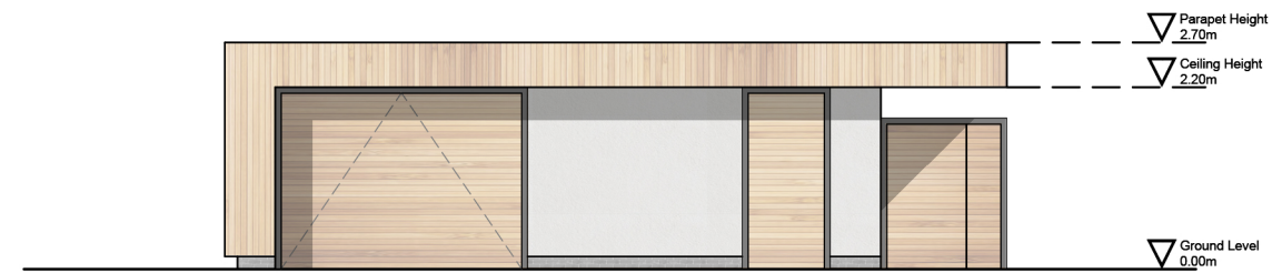
NORTH ELEVATION 1:100
