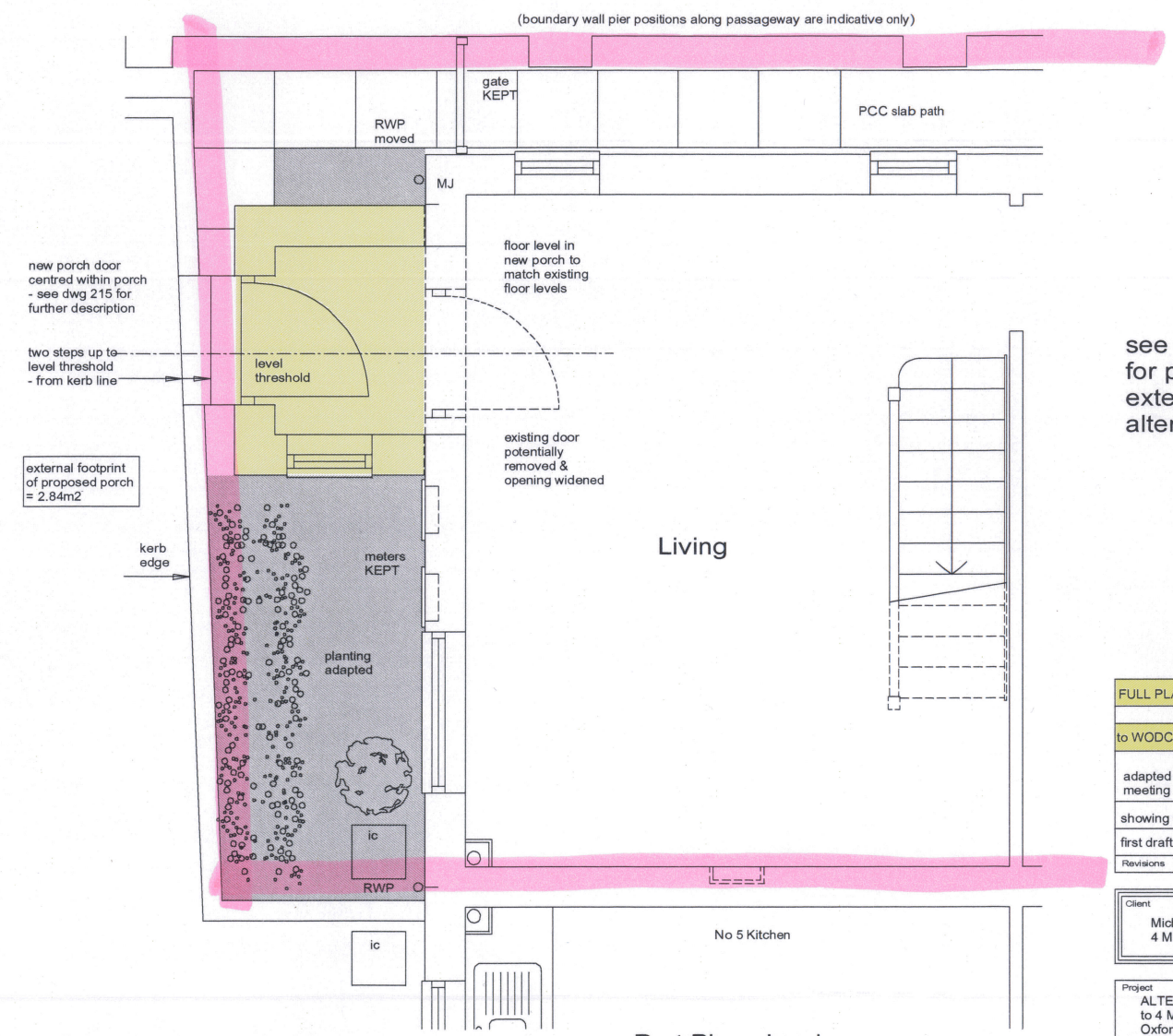
Part Plan showing Proposed Porch
