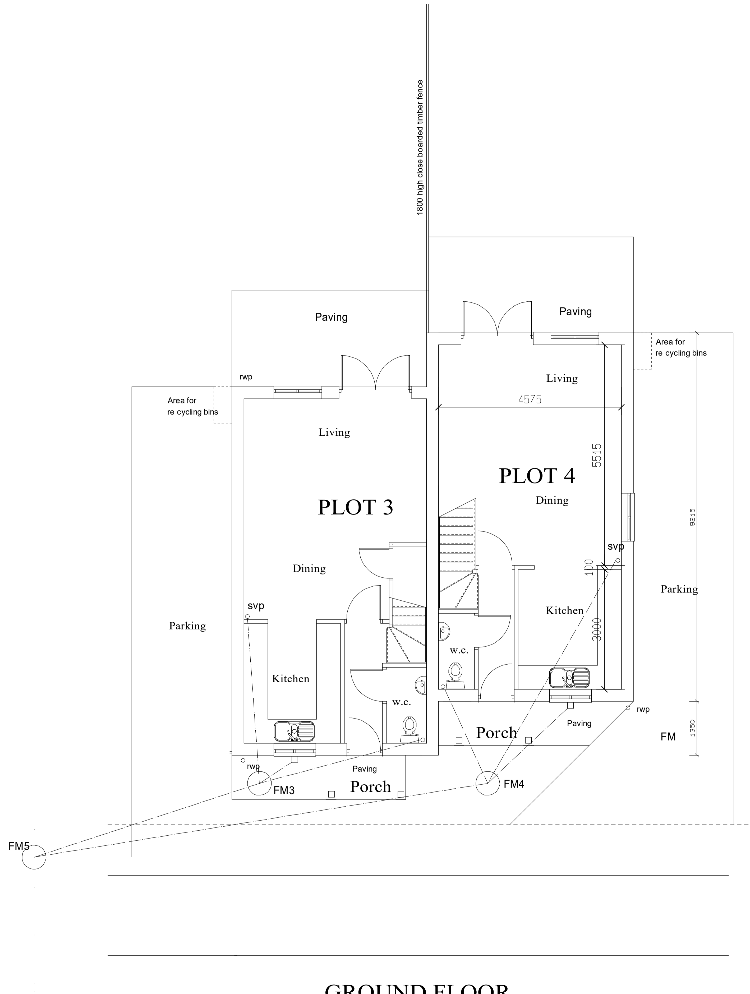
GROUND FLOOR
