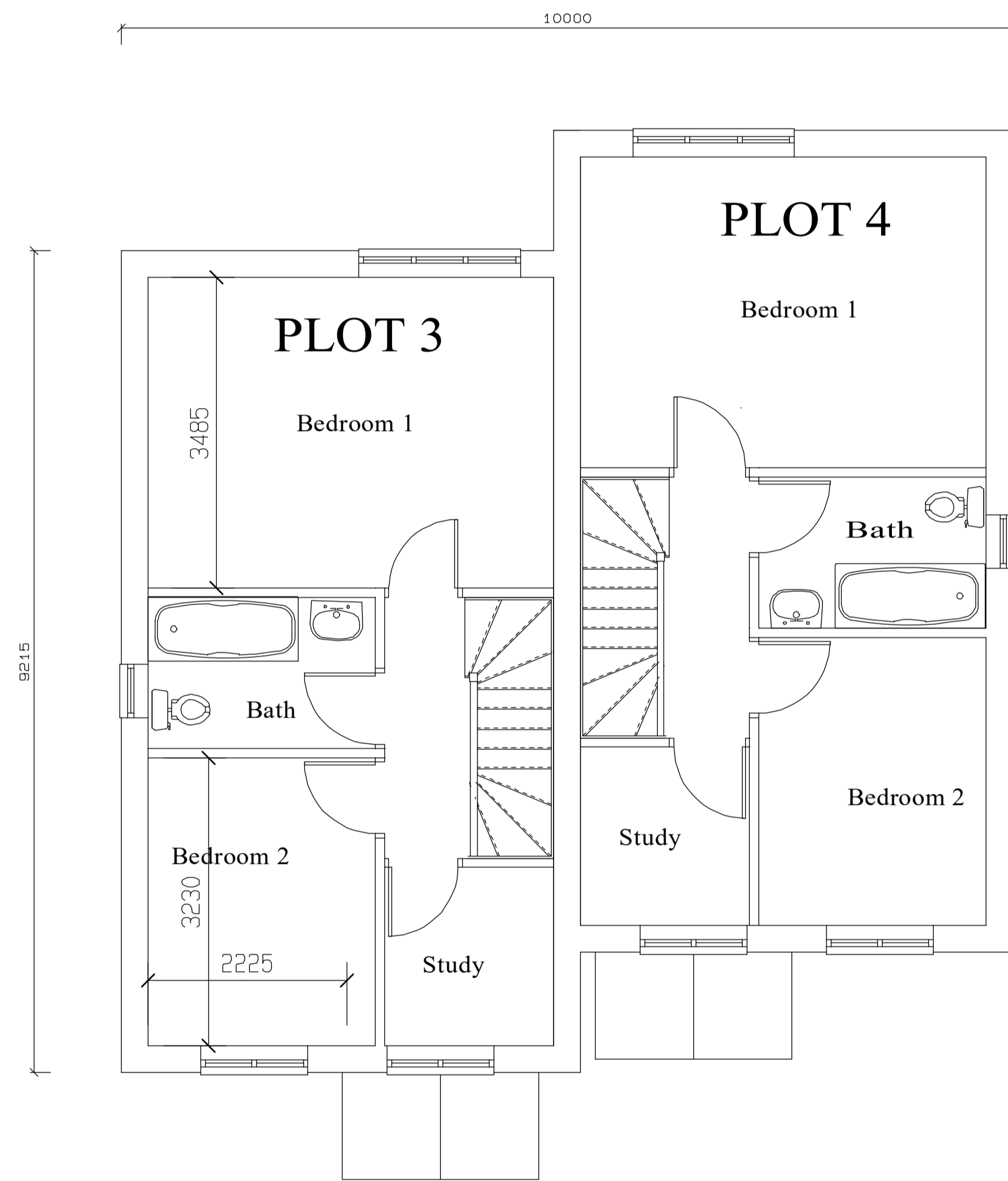
FIRST FLOOR
