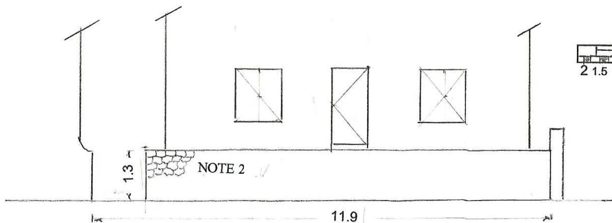
FRONT ELEVATION LOOKING NORTH EXISTING
